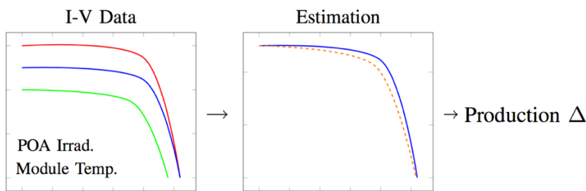
Figure 37: The Gaussian Process Regression algorithm was provided with I-V curve data to learn good system behavior. It then was provided with previously unseen irradiance and cell temperature inputs and estimated the ideal I-V curve.
